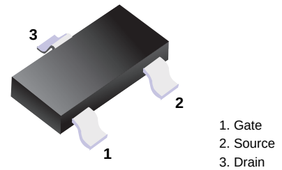
■ Simplified outline(SOT-23)
